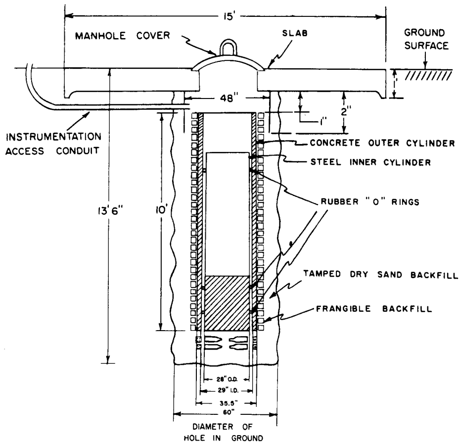
Fig. 7—Cross section of test structure in place.
